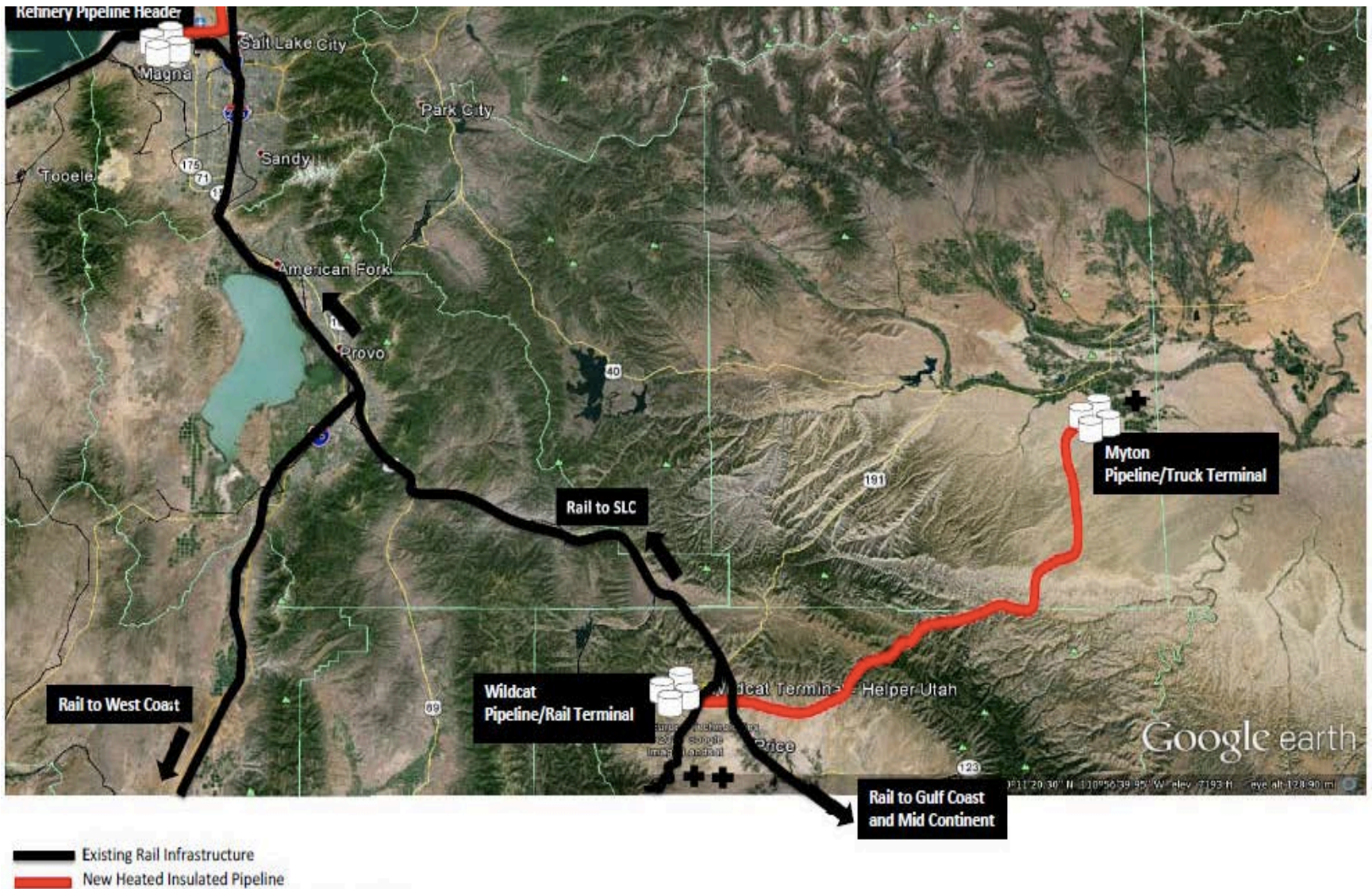
Pipeline and railroad route map from Azure Midstream.
